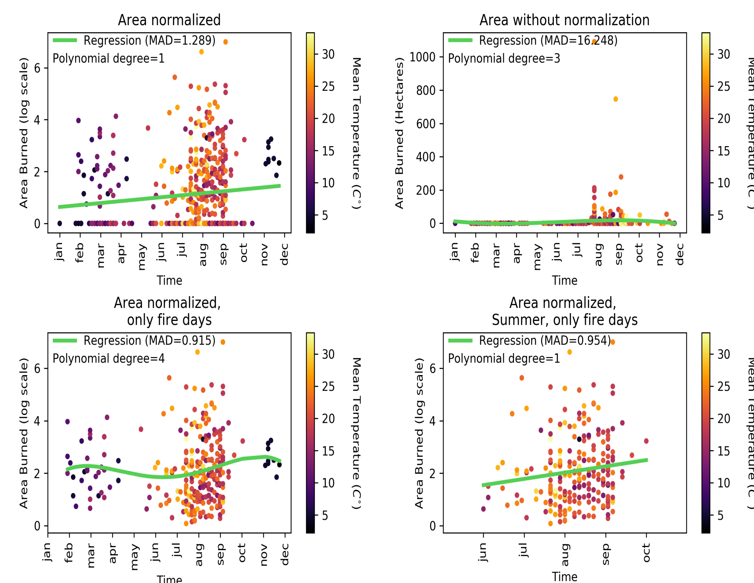
Area Burned at Various Individual Points in Time
